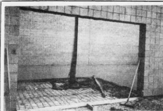
A flexible hose, suspended from giant overhead crane, depositing concrete in the section of the handball courts.
