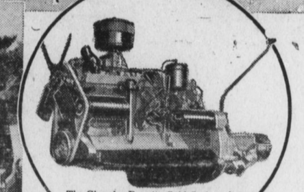
The Chrysler Royal's Gold Seal engine. This entirely new engine develops 93 h. p. with a piston displacement of but 228.1 cu. in.
