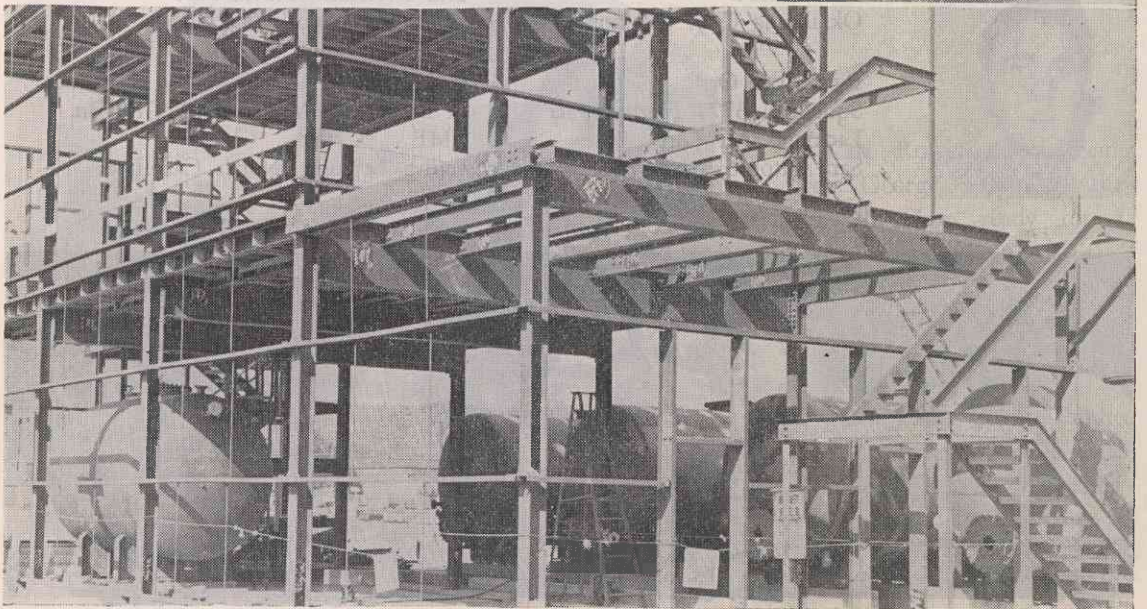
BELOW: Looking north at the structural steel and tank installations of the Solvent Recovery Building. In this building, evaporated solvents from the Coating Tower process will be recovered.
