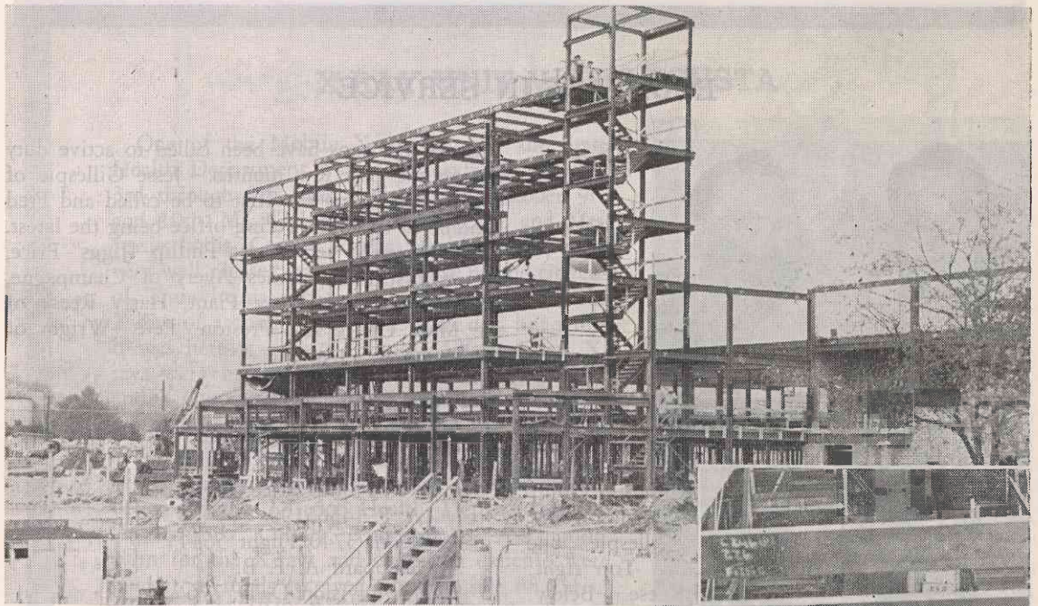
ABOVE: View showing Bath Mix House foundation in foreground and Coating Tower steel beyond.
