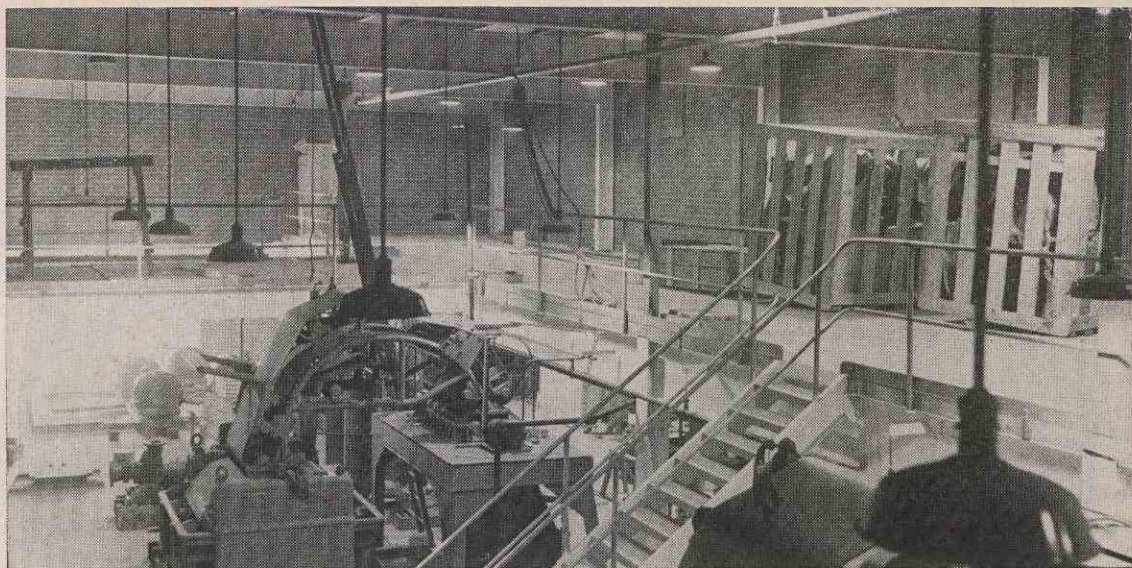
ABOVE: Continuous Steeping and Shredding units on 4th floor of Chemical House. Wood pulp feeders for these units are in the crates on upper level.
