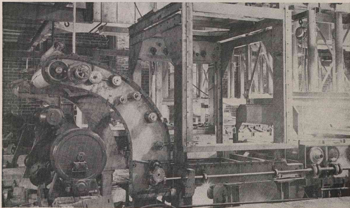
ABOVE: The wind-up end of No. 2 Casting Machine. Conditioner unit for adding moisture to the cellophane sheet will be located in box-like arrangement at right center.
