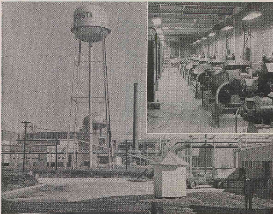
TOP RIGHT: Second floor of Casting Room. The motor-generators set and control the casting machine drives.
