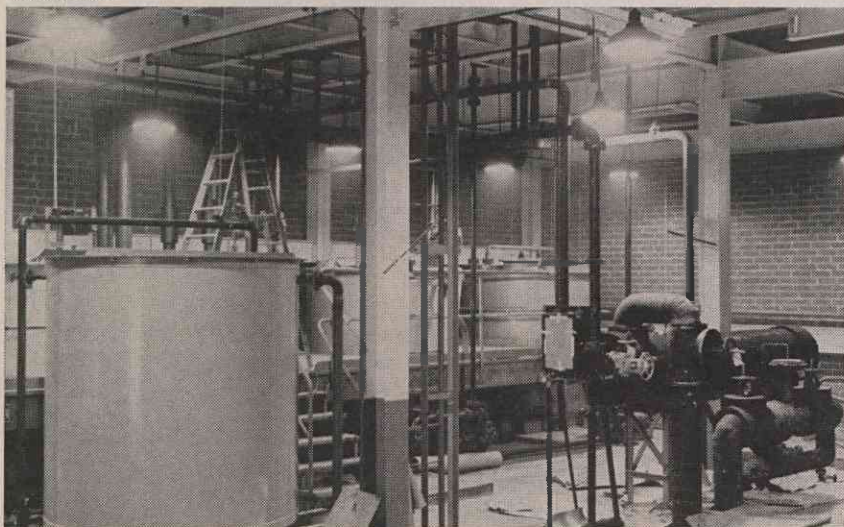
Second floor coagulating bath, showing caustic cooler and softener head tanks.
