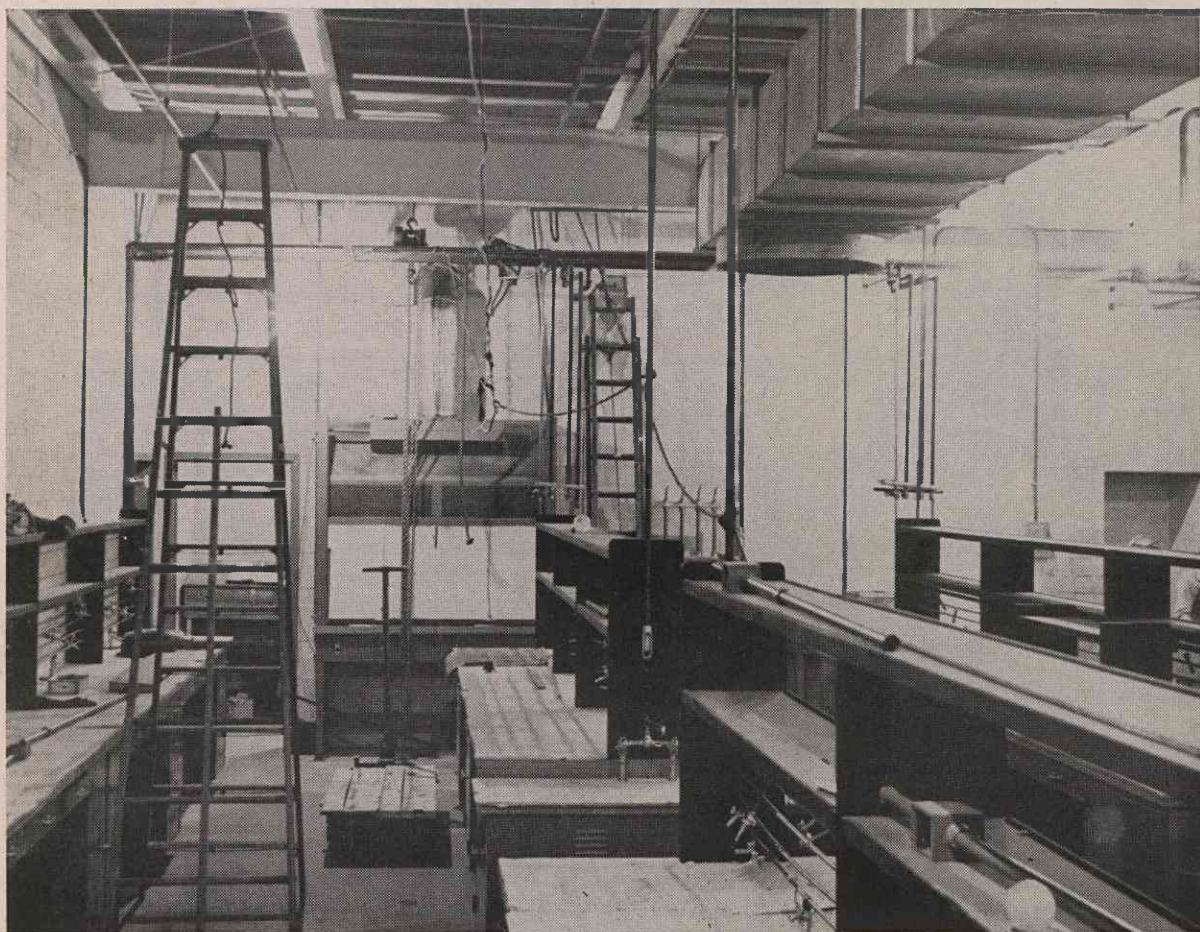
Hopper Repair Room, located on west side of Casting Room, showing surface grinder used to recondition casting machine hoppers.
