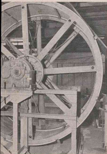
sheeting drum.
