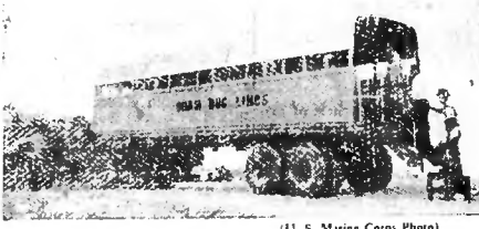
The 90-passenger bus used to transport Guamanians from their homes to jobs on important military installations was constructed from salvaged material by Marines and Seabees under the direction of Marine Maj. William J. Baker of Topeka, Kan., head of the island's military motor pool. The tractor part of the bus has been through the Bougainville and Guam campaigns; the trailer has considerable flap material in it. The bus is the first of several similar vehicles planned by the Civil Affairs Section of Marine Major General Henry L. Larsen's Island Command for civilians.
