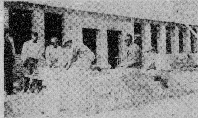
VET TRAINEES AT WORK — This building is being constructed by the Veterans of the Pikeville Training School bricklaying class under the supervision of Mr. Richardson.
