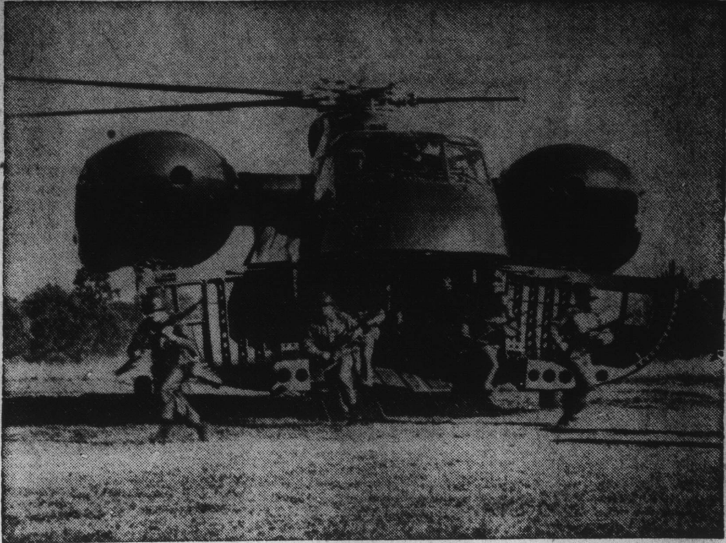
ARMY'S NEWEST —Air-lifted infantrymen charge from the clam-shell doors of the Sikorsky H-37 helicopter, the Army's largest, during a test maneuver at Fort Rucker, Ala. The twin-engine assault transport and cargo plane is being flight-tested by the Army Aviation Test Board. It can carry 33 fully equipped soldiers, compared with a limit of 20 in the largest Army plane now operational.
