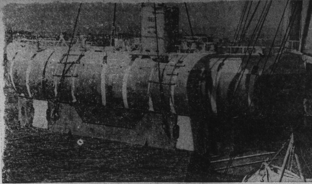
DOWN WE GO —With this blimp-shaped vessel, "Trieste," scientists hope to probe deeper yet into the ocean's canyons. Designed by French deep sea experts Auguste and Son Jacques Piccard, the device is being lifted onto a freighter at San Diego, Calif., for a voyage to the 35,000-foot Marianas Trench in the Pacific.
