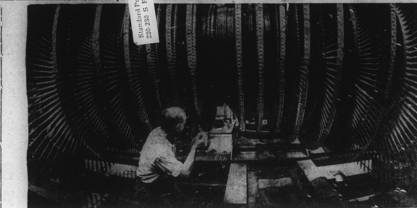
TURNING POINT—Painstaking care in the manufacture of large steam turbine-generators is apparent as this workman in Schenectady, N.Y., inspects one of the several thousand propeller-like buckets of this turbine rotor.
