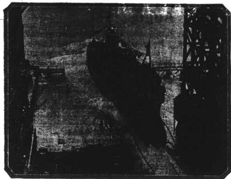
Photo of the launching at Portsmouth, N. H., Navy Yard of the U. S. Submarine, V-1, which is twice as large as any built previously for the U. S. Navy. The big undersea fighter is the first of a fleet of nine that will be able to accompany the battleships in any weather and at any speed of which the fleet itself is capable. The exact radius over which the V-1 can operate is not made known but it is hinted that it can cross the ocean and return without replenishing its fuel. The vessel is 341 feet, 6 inches, over all, has a maximum breadth of 27 knots and a speed of 9 knots submerged, and a surface displacement of 3,164 tons. She will carry a crew of seven officers and eighty men.
