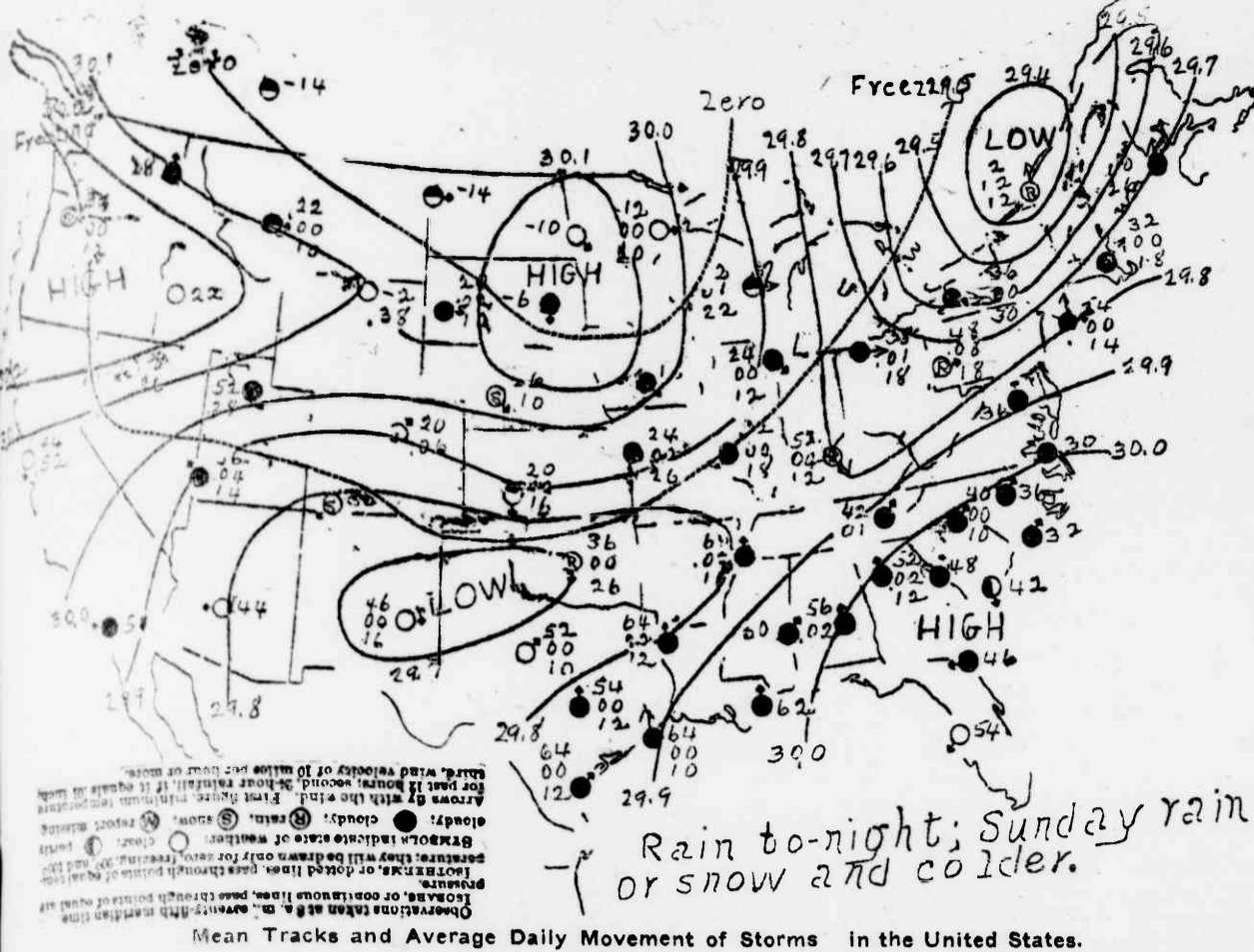
Mean Tracks and Average Daily Movement of Storms in the United States.
