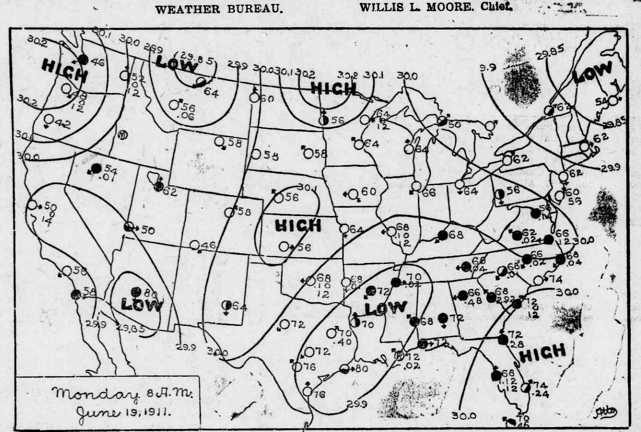
Observations taken at 8 a. m. 75th meridian time. Isobars or continuous lines, pass through points of equal air pressure. Isotherms, or dotted lines, pass through points of equal temperature.
