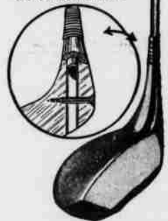
How the Bristol Steel Golf Shaft is Attached to the Wooden head
