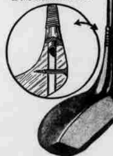
How the Bristol Steel Golf Shaft is Attached to the Wooden head
