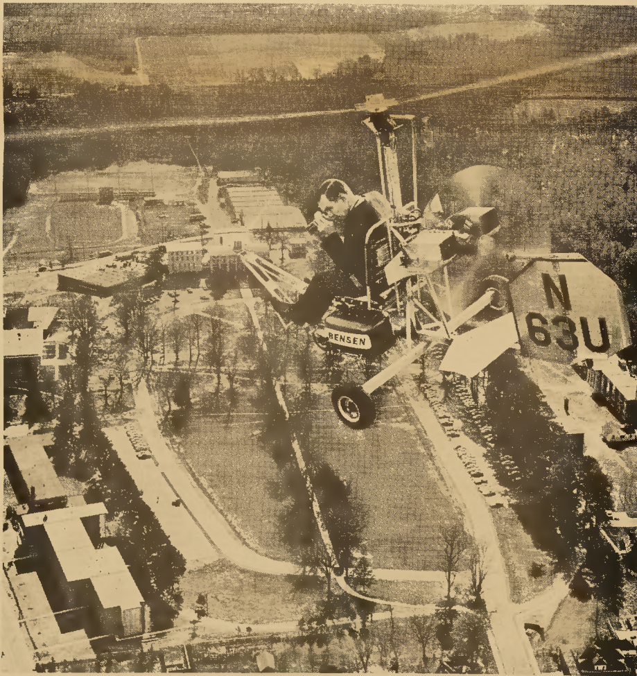
Single place gyrocopter by Bensen Aircraft Corp.
