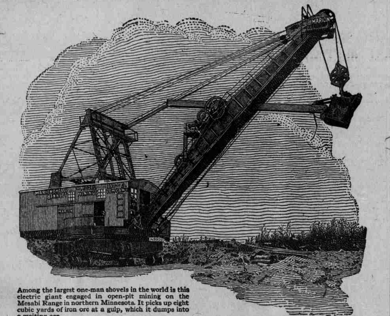
Among the largest one-man shovels in the world is this electric giant engaged in open-pit mining on the Mesabi Range in northern Minnesota.
