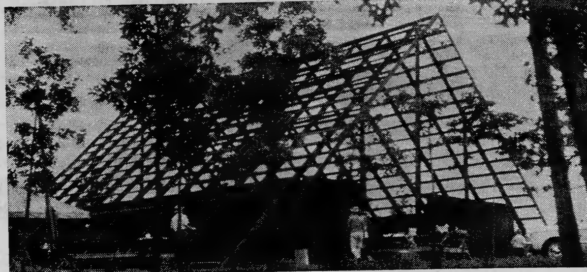
MOORE COUNTY WILDLIFE CLUB HOME, being constructed by the membership on a "pay-as-you-go" plan beside their lake on the old N'agata-Lakeview Road. The unique "A-frame" structure, 40 feet wide and 60 feet deep, was designed by Howard Butler, who is now club president. Rafters of 50-foot creosoted poles extend from ground to rooftop, 30 feet up. The lodge has no roof or floor as yet. Photo was taken while preparations were under way for a fish fry recently. (Photo by V. Nicholson)
