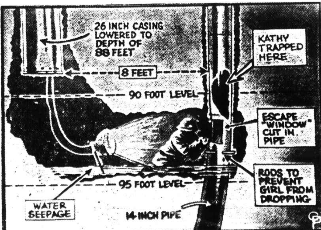
THIS DRAWING shows how rescuers finally approached the body of Kathy Fiscus. 3 and removed it from the steel-pipe tomb in San Marino, Calif. Pins were inserted at a point below where the girl was trapped to prevent her slipping down in case she were found alive. The top was said to have died soon after falling into the well. (International Soundphoto)
