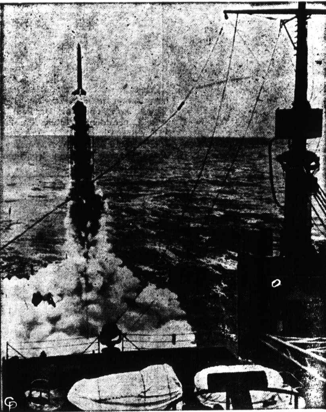
DURING A RECENT TEST, the Navy's guided missile, the "Aerobee," is headed skyward after being fired from the U.S.S. Norton Sound, somewhere in the North Pacific. The missile reached an approximate altitude of fifty miles. During most of the ascent, instruments in the nose of the "Aerobee" recorded cosmic ray research data, which was telemetered back to the experimental missile ship. (International Soundphoto)
