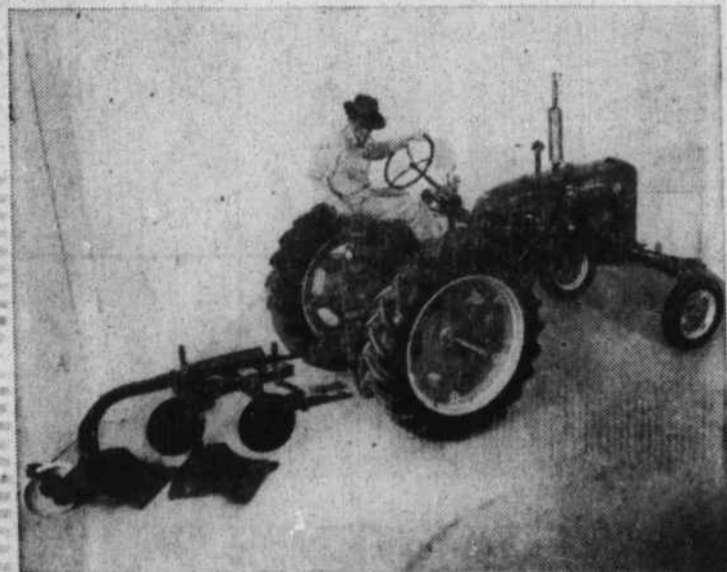
Here's how the new Farmall Fast-Hitch works; the farmer just backs up to the implement . . . the two coupling beams on the implement slip into the Fast-Hitch sockets on the tractor, and are locked instantly and automatically—to uncouple, just lift two latches. The farmer saves a great deal of time and all of the hard work usually required in hitching.
