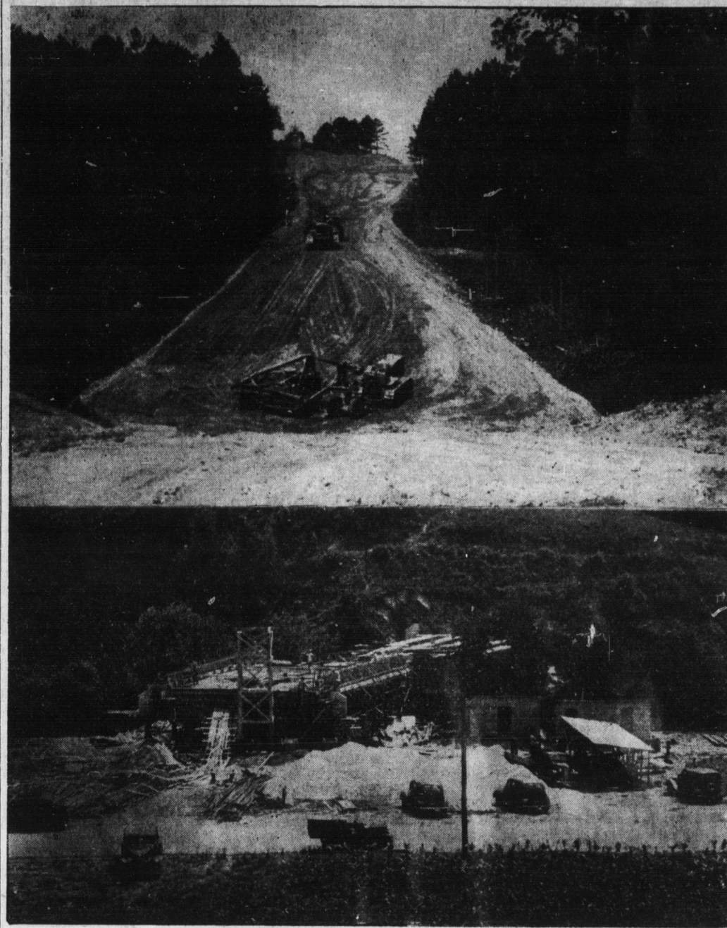
The task of grading the right-of-way for the new western approach to Elkin of route 268, is showing fast progress as huge scoops, capable of moving 12 yards of dirt at a load, bite into the hills. Top photo, made on the new roadway, facing west toward the intersection of 268 with the Traphill road, shows the work of grading in progress. Bottom photo is view of bridge being constructed across Big Elkin creek near the old shoe factory.—(Tribune Photos.)
