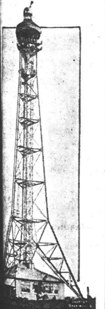
At the "hitching post" at the wharf hangar to which the largest airship, the U. S. Shenandoah, is to be moored.
