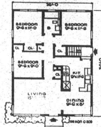
A SMALL HOUSE PLANNING BUREAU DESIGN NO. C-309
