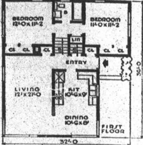
A SMALL HOUSE PLANNING BUREAU DESIGN NO. C-310-S
