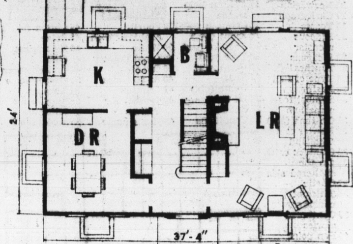
PLAN NO. 7179 CENTER SECTION SCALE IN FEET
