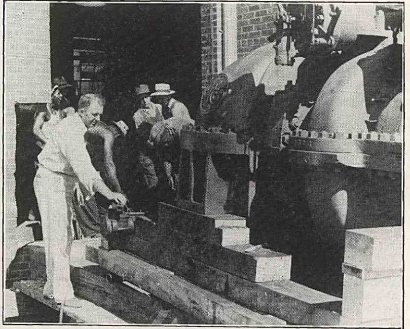
Top photo shows Mr. Morgan supervising the unloading of our new steam turbine that has been installed at the power plant and is now in operation. This machine is carrying the whole load of the entire mill at the present time.
