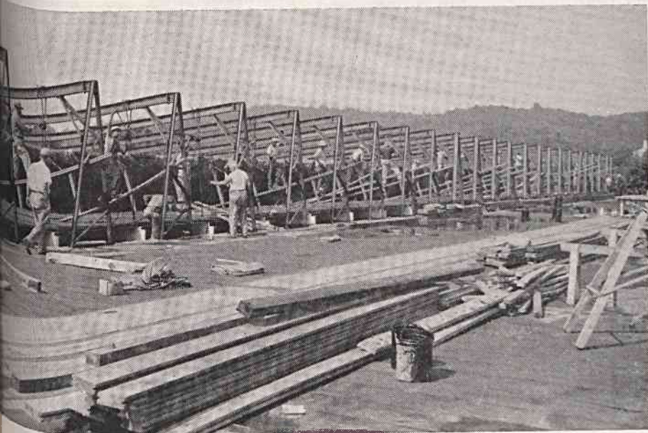
Workmen lower a section of the old saw-tooth roof at the Towel Mill to make ready for a modern, insulated roof in connection with evaporative cooling system.
