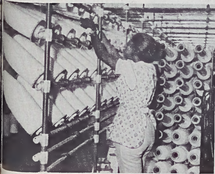
Twister tender creels in new bobbin on twister.
