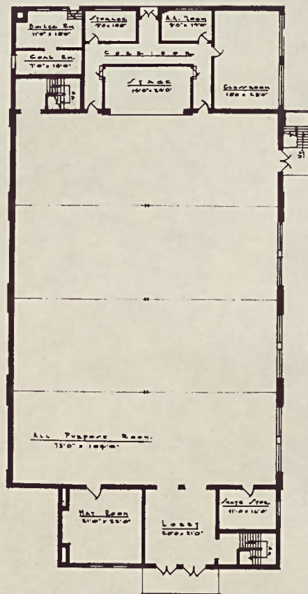
GROUND FLOOR PLAN SCALE 1/8" = 1'-0"
