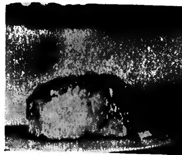
MUG SHOT . . . This is a closeup view of Apollo 15 lunar sample No. 15415 at the Manned Spacecraft Center. This sample is the white anorthositic rock ("Genesis rock") collected by Astronauts David R. Scott and James Irwin on the mission's second extravehicular activity.
