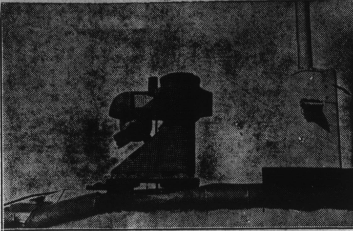
SNORKEL (BREATHING DEVICE) ON GERMAN SUBMARINE —This breathing device was used by the Germans in latter stages of World War II, permitting their submarines to patrol continuously submerged. Diesel gases are exhausted and fresh air received via an opening above the "float valve" near the top of the snorkel. The wire mesh encasement was intended to reduce possibility of radar detection. At the right is the periscope, shown extended.
