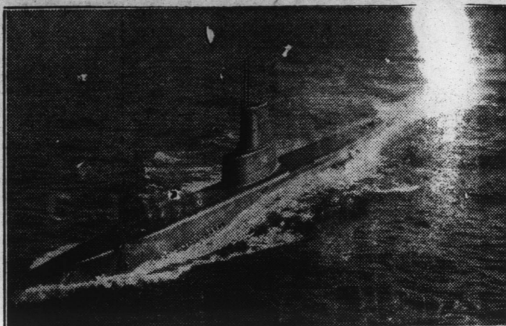
USS CORPORAL (SS 346), A CONVERTED U.S. FLEET TYPE SUBMARINE —Conversion of this submarine to a Guppy-type was accomplished by superstructure stream-lining and increasing battery capacity to give greater submerged speeds. The name "Guppy" stems from the name of the conversion program—Greater Underwater Proposed Propulsion. Approximately 24 U.S. fleet type submarines have been converted to the Guppy class.
