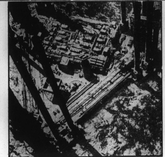
"EYES OF TEXAS" ARE UPON THEM —This is a helicopter-view of a "Texas Tower" being floated into position near Georges Banks in the Atlantic Ocean off the coast of Cape Cod. It will serve as a man-made island to house radar equipment as part of the nation's air-raid warning net. Developed originally for use in drilling for off-shore Texas oil, the island is secured in position by jacking the smokestack-like tubes at each corner of the triangular island down to the sea floor.
