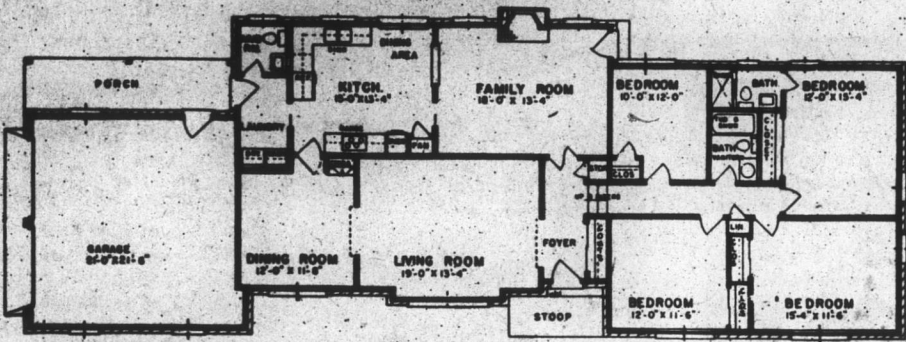
DRYSDALE PLAN No. 4-X, Overall Dim. 92'-10", House 2,059 Sq. Ft. In B. V., Garage, Porch & Stoop 676 Sq. Ft.
