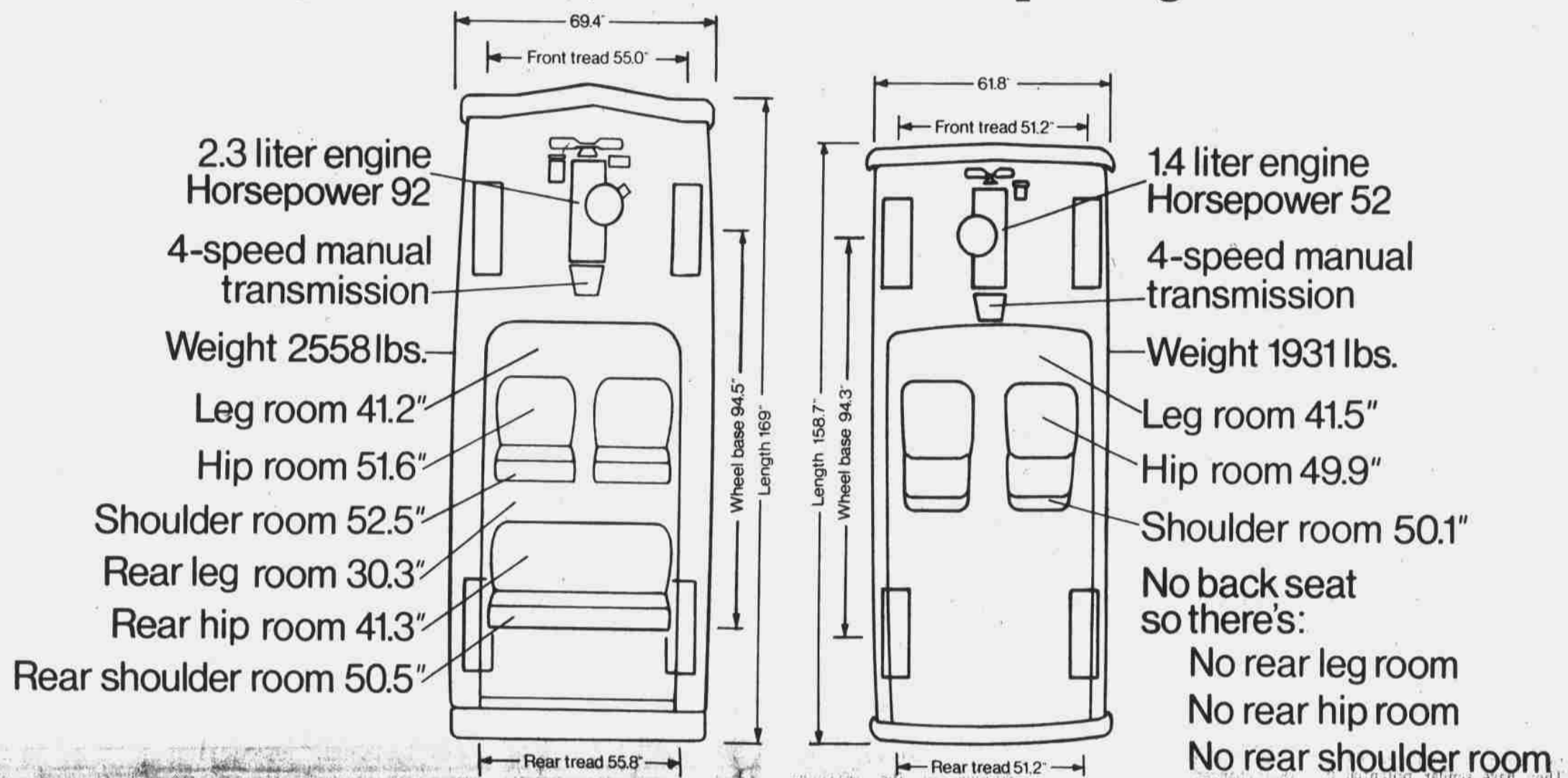
The 2-passenger Chevette Scooter
