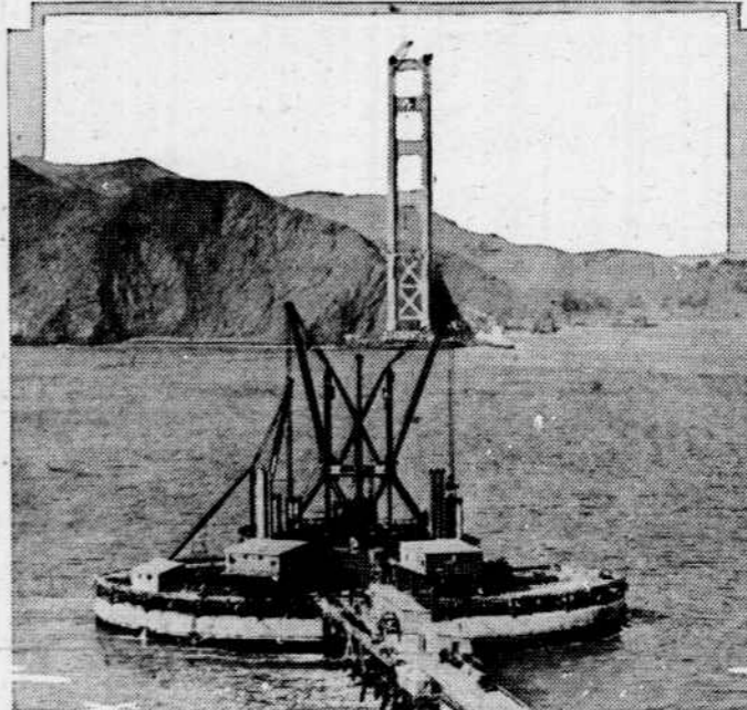
A new and spectacular landmark has commenced to take form at San Francisco's harbor entrance. It is the south tower of the Golden Gate bridge that, with its twin on the Marin side of the Golden Gate, will support the world's greatest suspension span. Already the first sections of tower steel, some of the units of which weigh 70 tons, have been erected and approximately 1,500 tons of fabricated material are on the loading platform on the south pier fender in readiness to be erected. Photograph shows the south tower of the Golden Gate bridge. In the distance can be seen the north tower on the Marin side.
