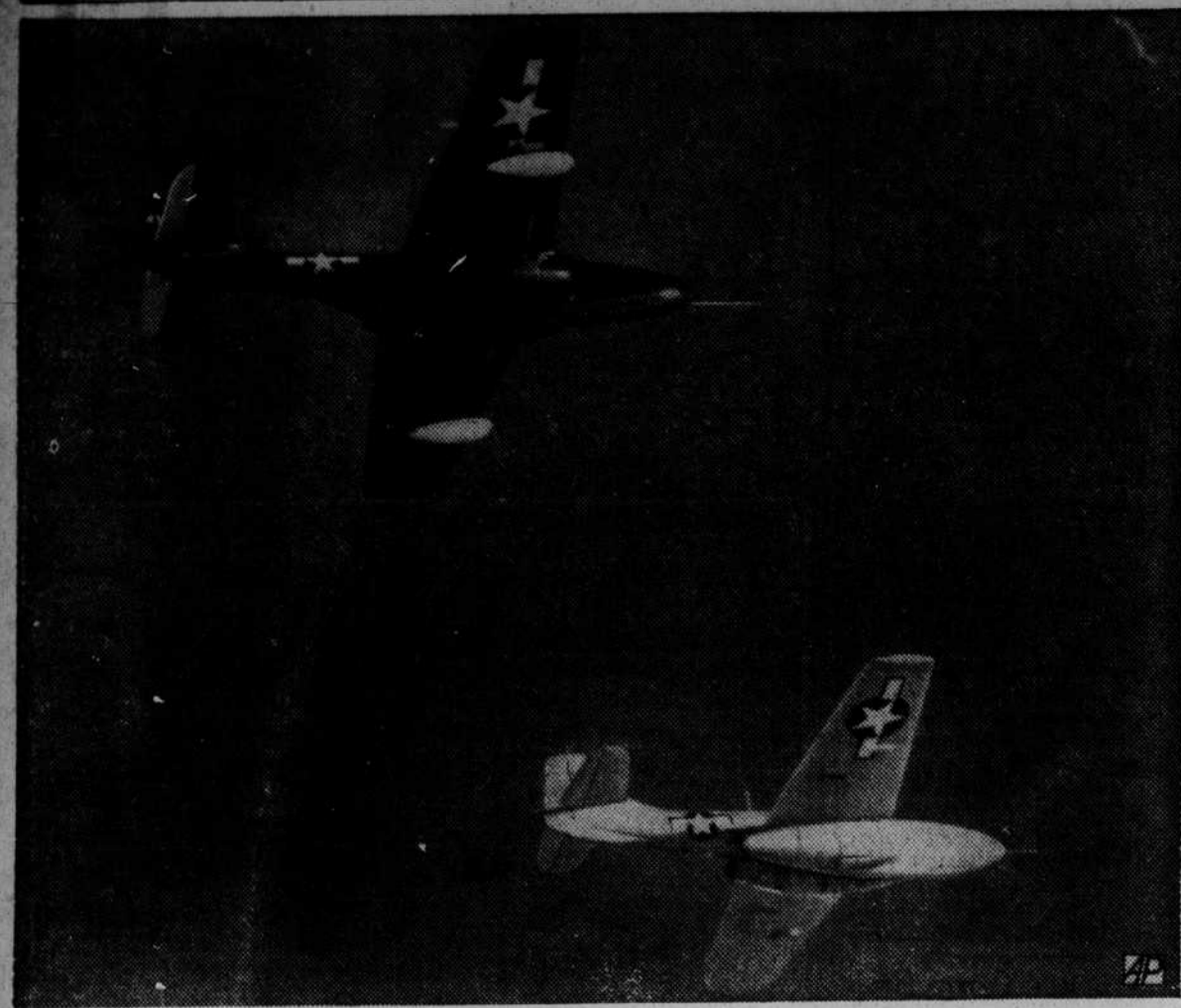
JET PLANE AND 'MOTHER' SHIP—Two jet-propelled P-59 Aircromets in the radio remote control aircraft project developed by the Air Technical Service Command and Bell Aircraft Corporation are shown in test flight over a field at Niagara Falls, N. Y. At top is the "mother" or control ship, and below the controlled or "robot" aircraft.
