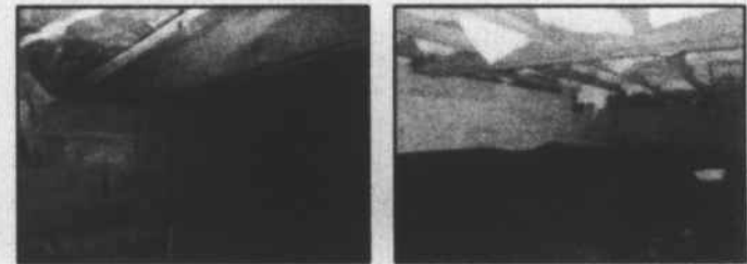
Addition of Floor Insulation and Vapor Barrier: Missing or deteriorated insulation is replaced with R19 fiberglass batts ground covered with vapor barrier to prevent mold and moisture.
