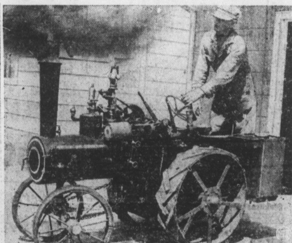
NEW OLD-TIMER—John E. Peters, retired farmer of Inman, Kan., steers the pint-sized reproduction of an old-time Rumley steam thrasher machine tractor which he made from scrap and junk. Coal is used to fire the boiler and with full steam up, the thrasher will move about four miles per hour. The whistle, governor, steering wheel and wheels were made from old tractor parts; the boiler from oilfield pipe; smokestack, coal and water bins from tin, and tires and belts from salvaged tires and tubes. Peters' hobby is making models of outdated farm machinery. EXCLUSIVE NEA PHOTO.
