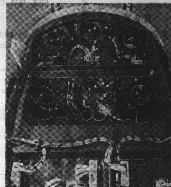
RANGER'S "EYES"—Close-up photo shows the six television cameras that will allow NASA's Ranger-B to take pictures of the moon.
