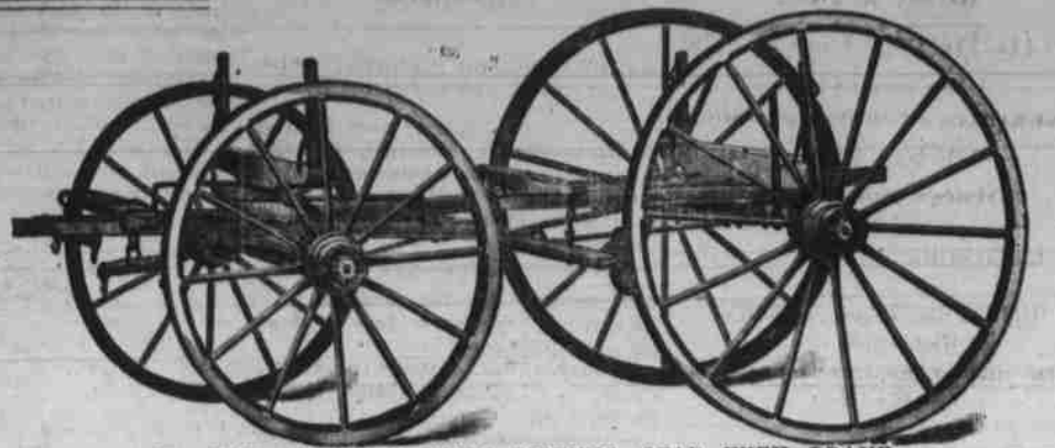
3x9" CAST THIMBLE SKEIN RUNNING GEAR WITH BRAKE.
