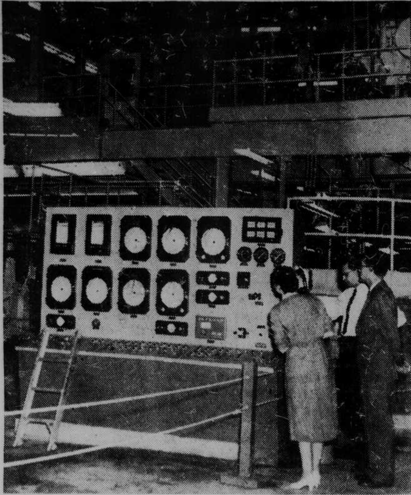
HUNDREDS OF TRANSYLVANIANS inspected the new "Cherokee Arrow", the largest paper machine in America for the manufacture of lightweight paper, at the Ecusta Paper division of the Olin Mathieson Chemical corporation at Pisgah Forest last Friday night. In the left photo Ray Hooper, quality control manager, and Edgar Loftis, assistant to the production manager, explain the machine operator's panel to a visitor. In the picture above Marcy Newell, process engineer, tells of the operations of the stock prep panel to a group. The three refiner beaters of the new No. 10 paper machine can be seen at the right, as they are inspected by visitors and plant officials. (Photos by Russell and Anderson)
