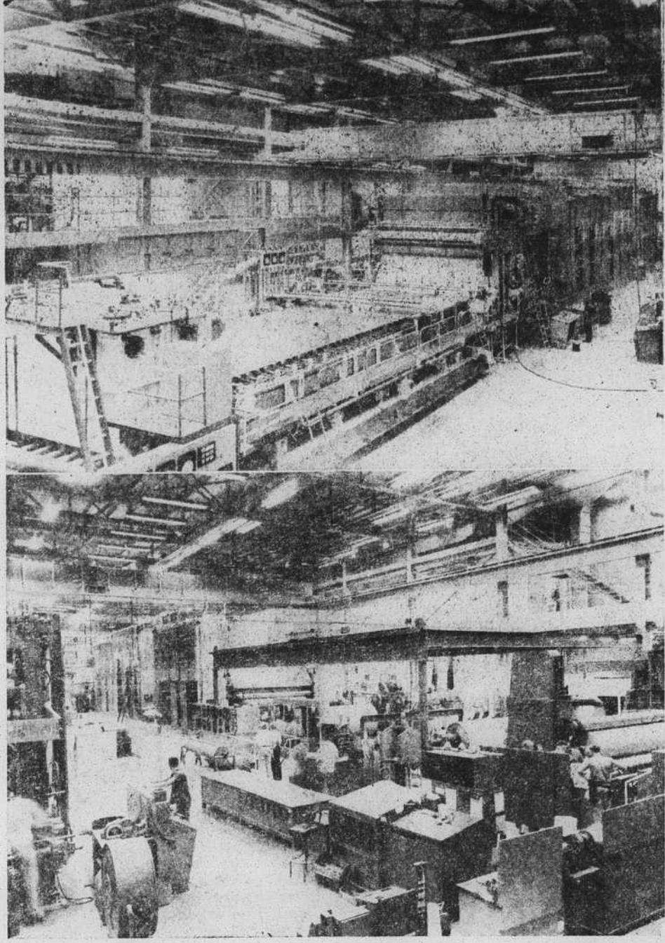
THE FIRST SHEET OF PAPER on Ecusta's No. 11 paper machine, which is recognized as the world's most modern for the manufacture of lightweight paper, is pictured in the top photo. The photograph beneath shows the dry end of the paper machine and the rewinder.
