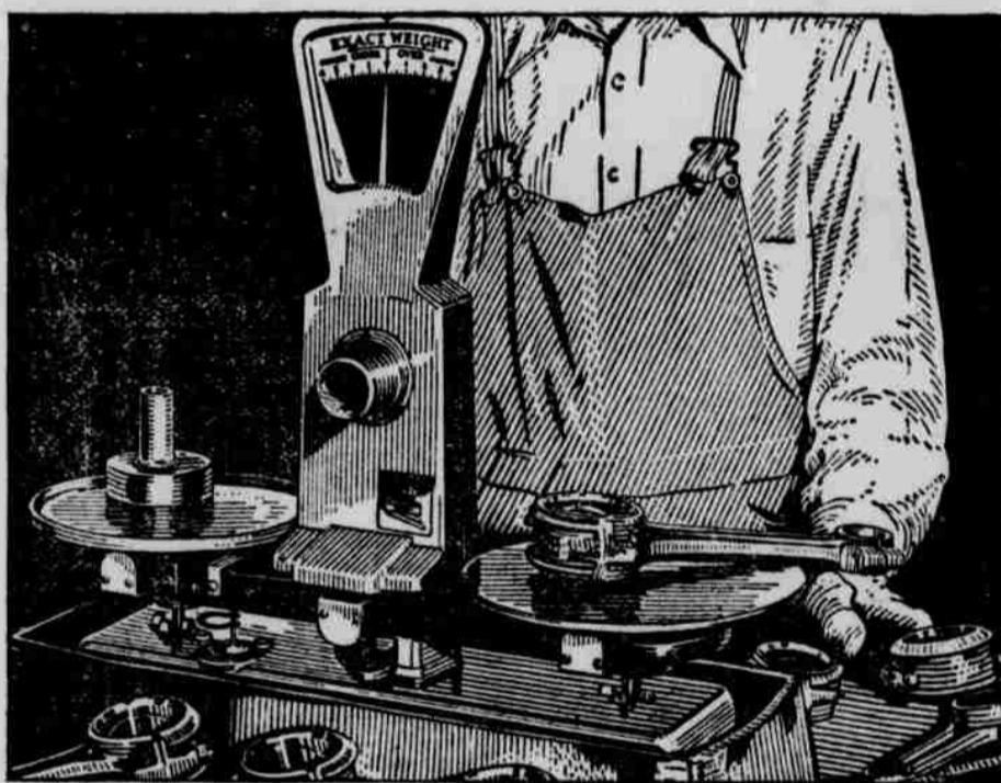
Chevrolet connecting rods are matched in sets of six to within one-quarter ounce, and are individually fitted by hand to the crankshaft. Bearings are of Bobbitt metal cast into the rods under heavy air pressure and at 800° Fahrenheit.
