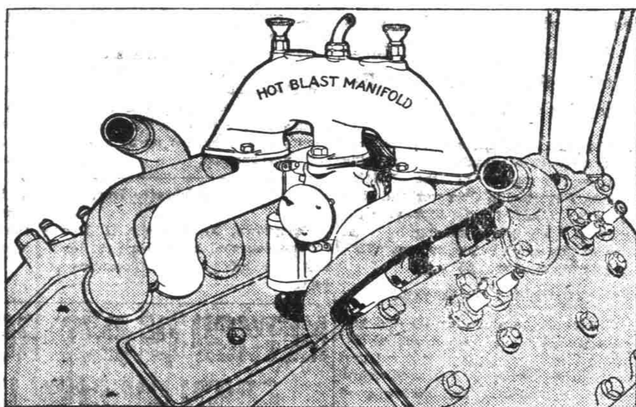
Aero-EIGHT Hot-Blast Manifold Assembly
