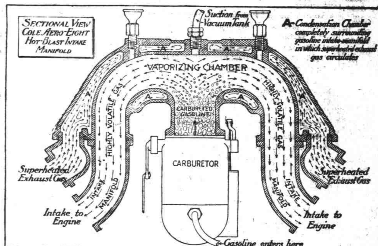
Operation of Aero-EIGHT Hot-Blast Manifold
