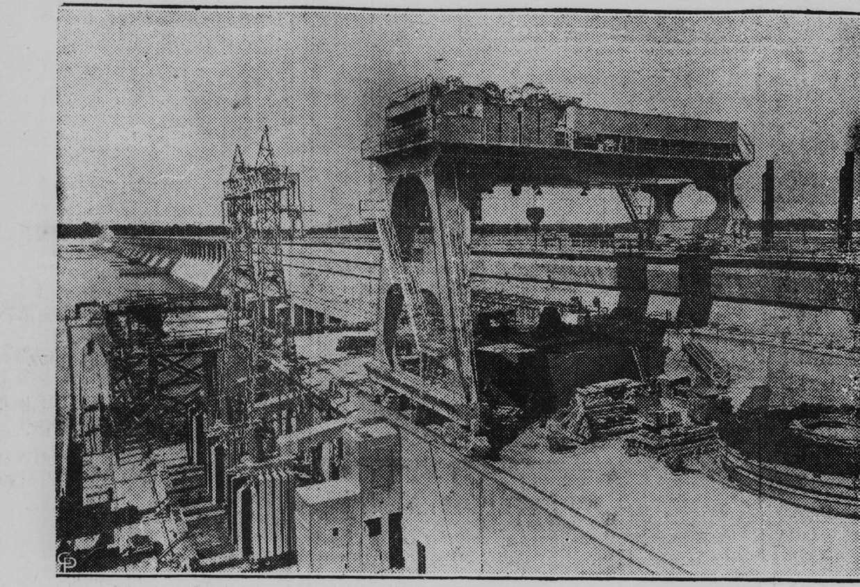
Installation of one of the two 45,000-horsepower generating units at the Wheeler dam on the Tennessee river, above, marks another important step in the progress of the vast TVA power program. —Central Press
