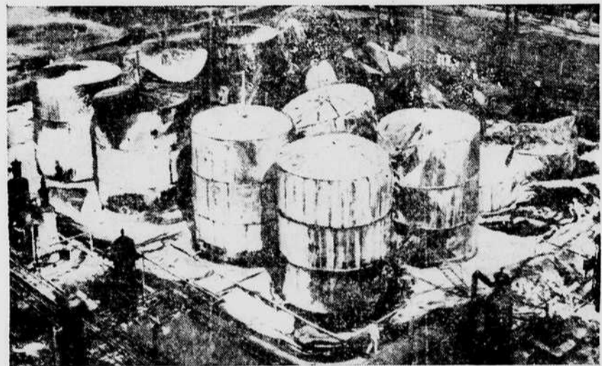
INTENSE HEAT of blasts and fire at Inglewood, Cal., leaves storage tanks crinkled, shrunken.
